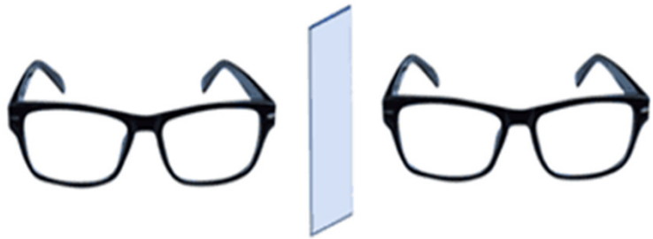
achiral - superimposable
